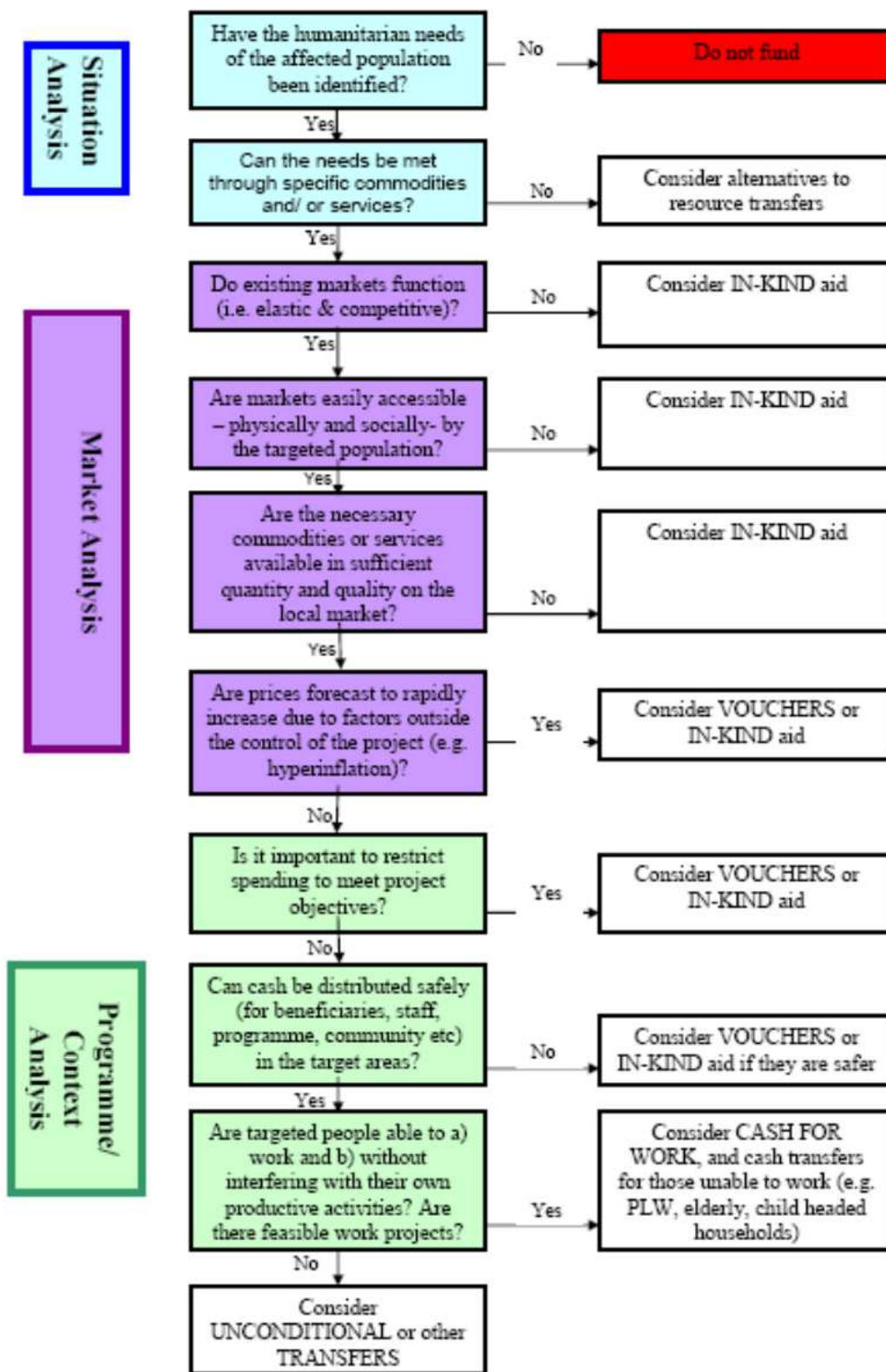
Figure 1 Decision tree
